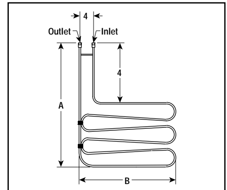
US4 — Dimensions (Inches)
