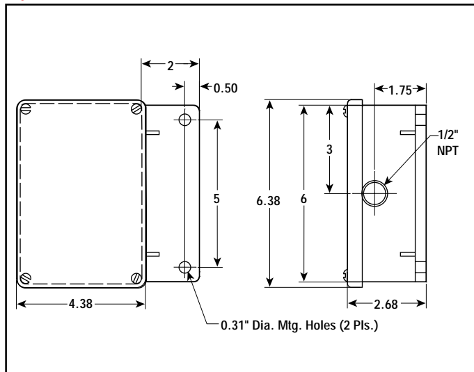
Style E — Dimensions (Inches)
