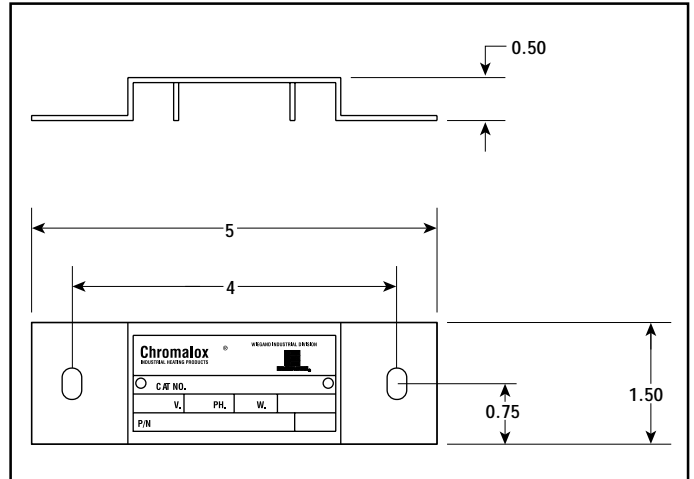
Style B — Dimensions (Inches)
