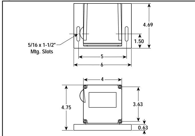
Style C — Dimensions (Inches)
