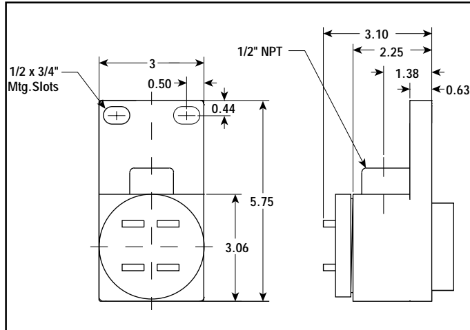
Style A — Dimensions (Inches)
