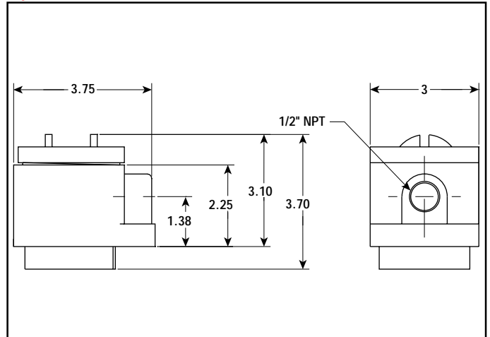
Style D — Dimensions (Inches)
