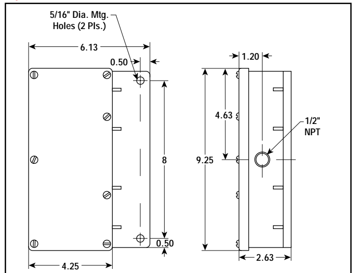
Style F — Dimensions (Inches)
