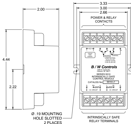
5510 SERIES RELAY INTRINSICALLY SAFE
