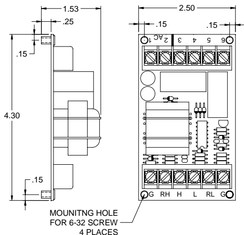
5500 SERIES RELAY NON-INTRINSICALLY SAFE
