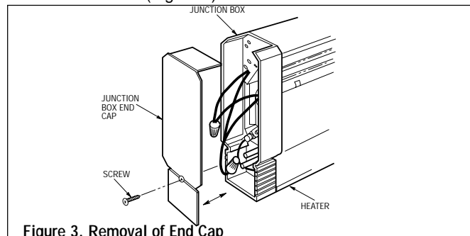
Figure 3. Removal of End Cap
