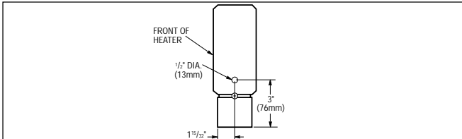
Figure 9. End Cap Drill Pattern
