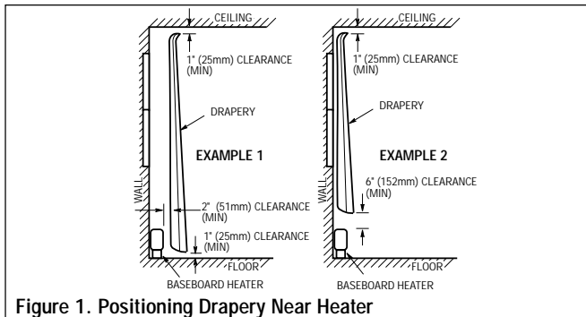
Figure 1. Positioning Drapery Near Heater
