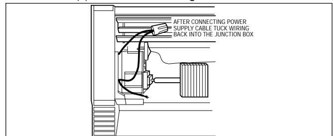
Figure 8. Wiring Through Junction Box Opening
