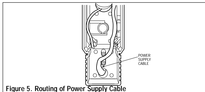
Figure 5. Routing of Power Supply Cable
