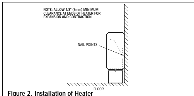
Figure 2. Installation of Heater
