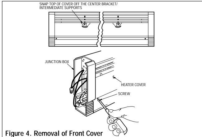
Figure 4. Removal of Front Cover
