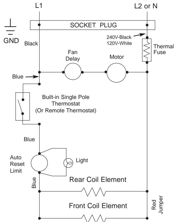
Wiring Diagram - Toe Space Heater For lower wattage rating, remove red jumper
